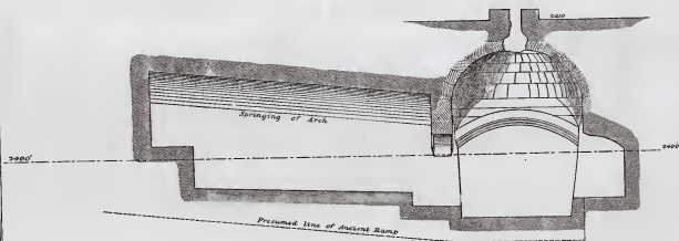
Scale 1/2" SECTION ON A.B.
